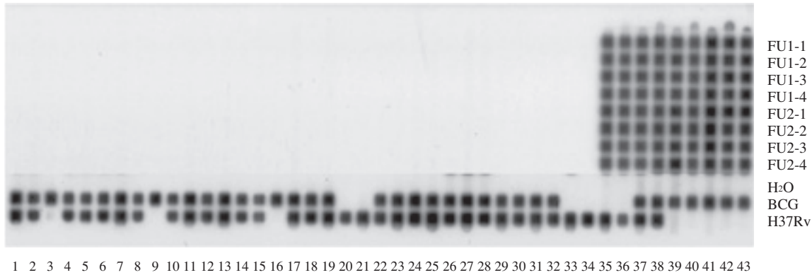
Fig. 2 Hybridization patterns (spoligotypes) from clinical strains of MDR-TB in this study, M. bovis BCG, and M. tuberculosis H37Rv. A membrane with 43 spacer oligonucleotides was used (vertical lines). The spoligotype of the clinical strains of MDR-TB corresponds to that of strains from the described Beijing genotype group.
