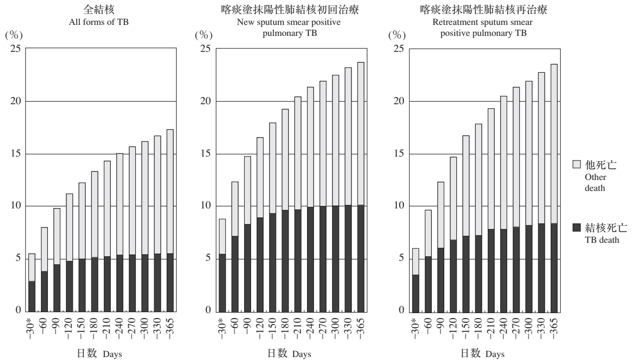
図2 2008年新登録結核患者中治療開始後1年以内死亡者の時期別累積死亡割合 Fig. 2 Cumulative proportion of deaths among newly notified TB patients in 2008 by period from the beginning of treatment -30*: 死亡後登録・治療前死亡を含む including cases who died before the beginning of treatment
